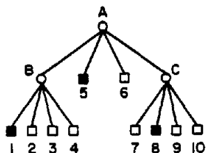
Figure 19. Sample image and its quadtree.
