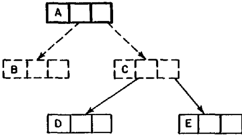
Figure 52. Strip tree corresponding to Figure 51.
