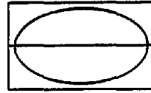
Figure 53. Modeling a closed curve by a strip tree.
