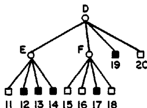
Figure 20. Sample image and its quadtree.
